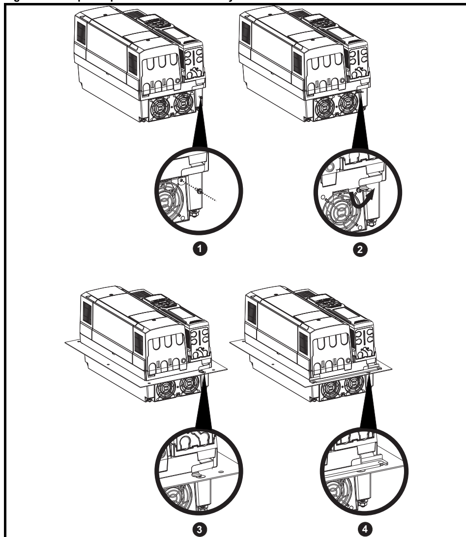
Figure 3-16 Special procedure for size 7 only
