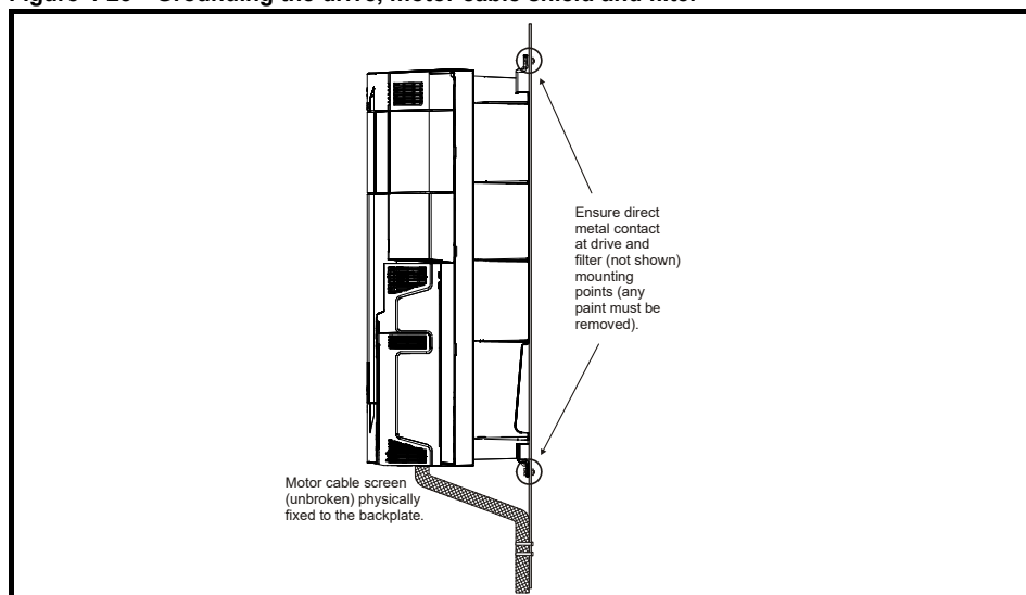
Figure 4-23 Grounding the drive, motor cable shield and filter
