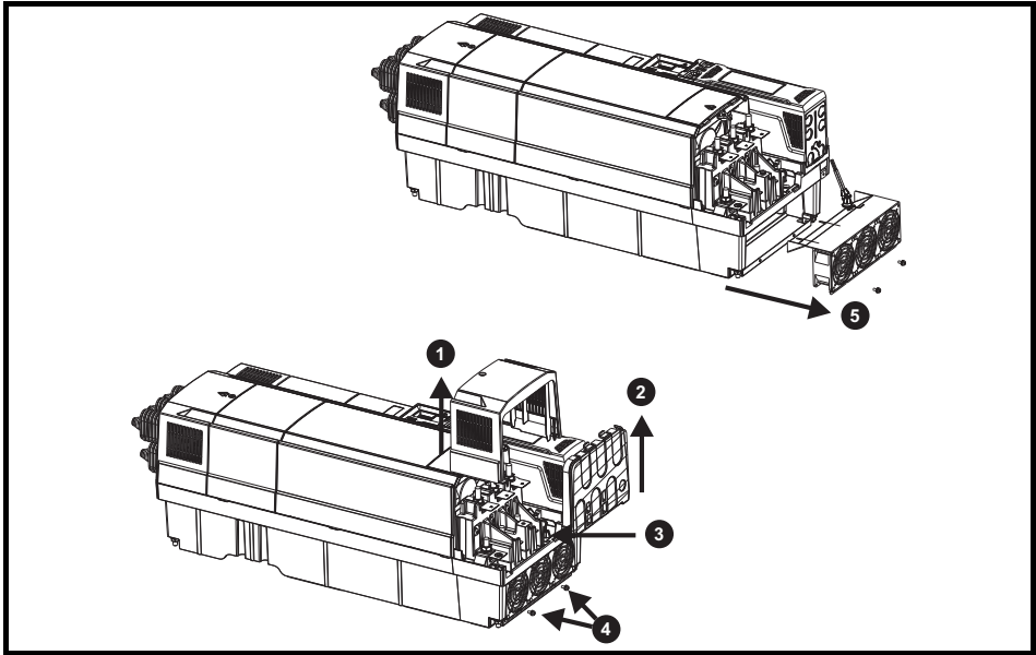
Figure 3-25 Size 8 heatsink fan replacement
