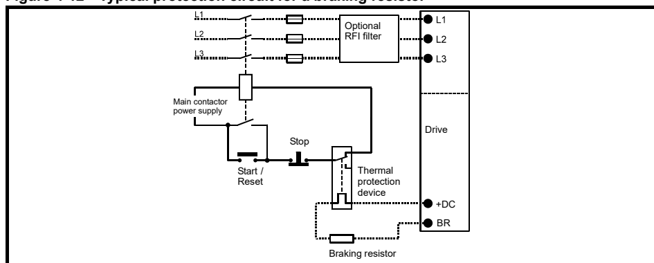
Figure 4-12 Typical protection circuit for a braking resistor
