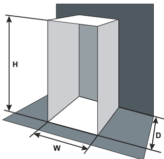
Figure 3-14 Enclosure having front, sides and top panels free to dissipate heat
