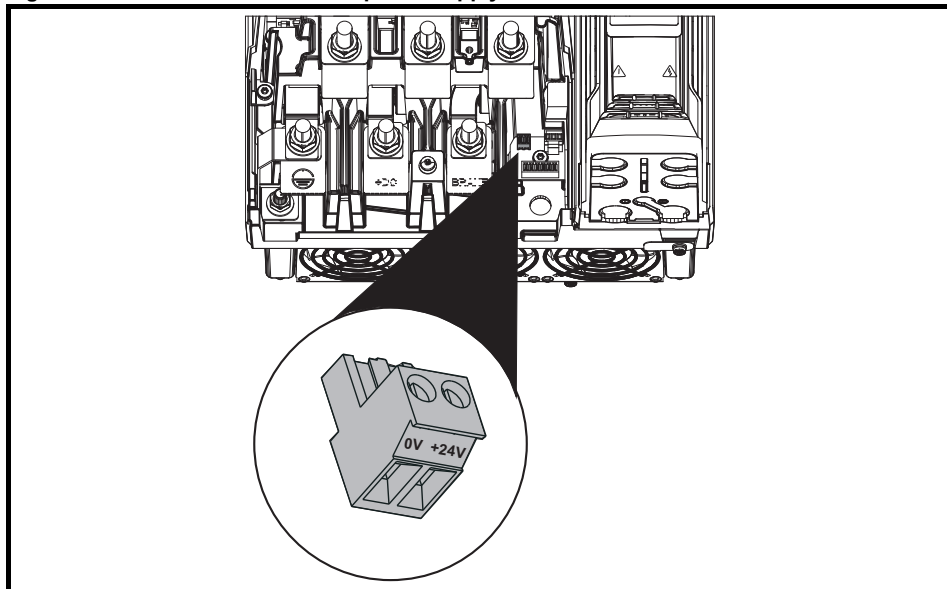
Figure 4-7 Location of the 24 Vdc power supply connection on size 8 to 10
