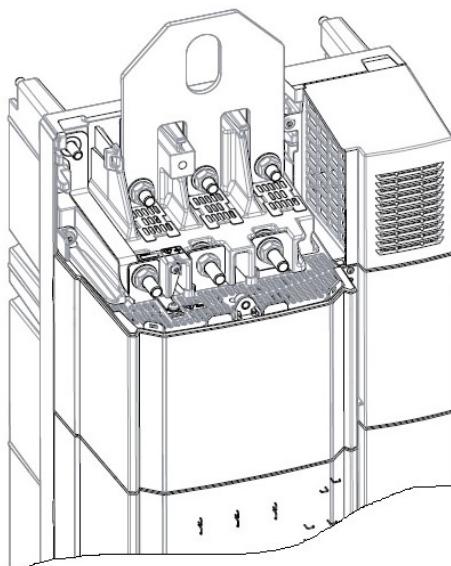
Size 11E/T and size 11 single/twin Rectifier Lifting tool 7778-0030
