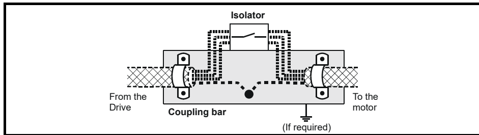
Figure 4-28 Connecting the motor cable to an isolator/disconnect switch
