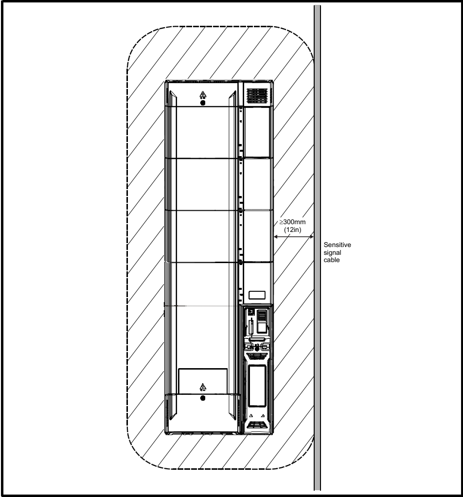
Figure 4-22 Sensitive signal circuit clearance
