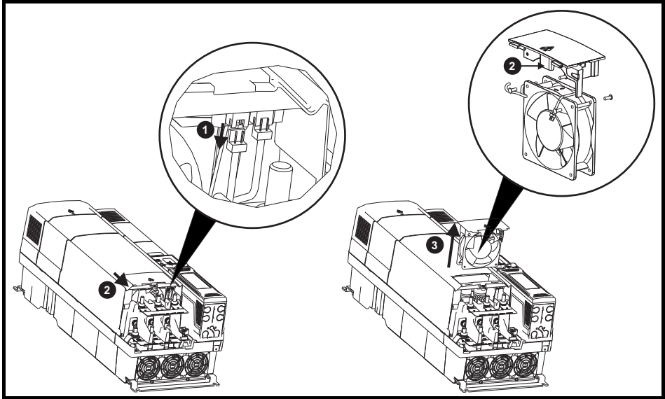
Figure 3-27 Size 7 to 10 auxiliary (capacitor bank) fan replacement
