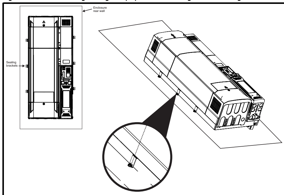
Figure 3-19 View showing sealing clamps provided in through hole mounting kit
