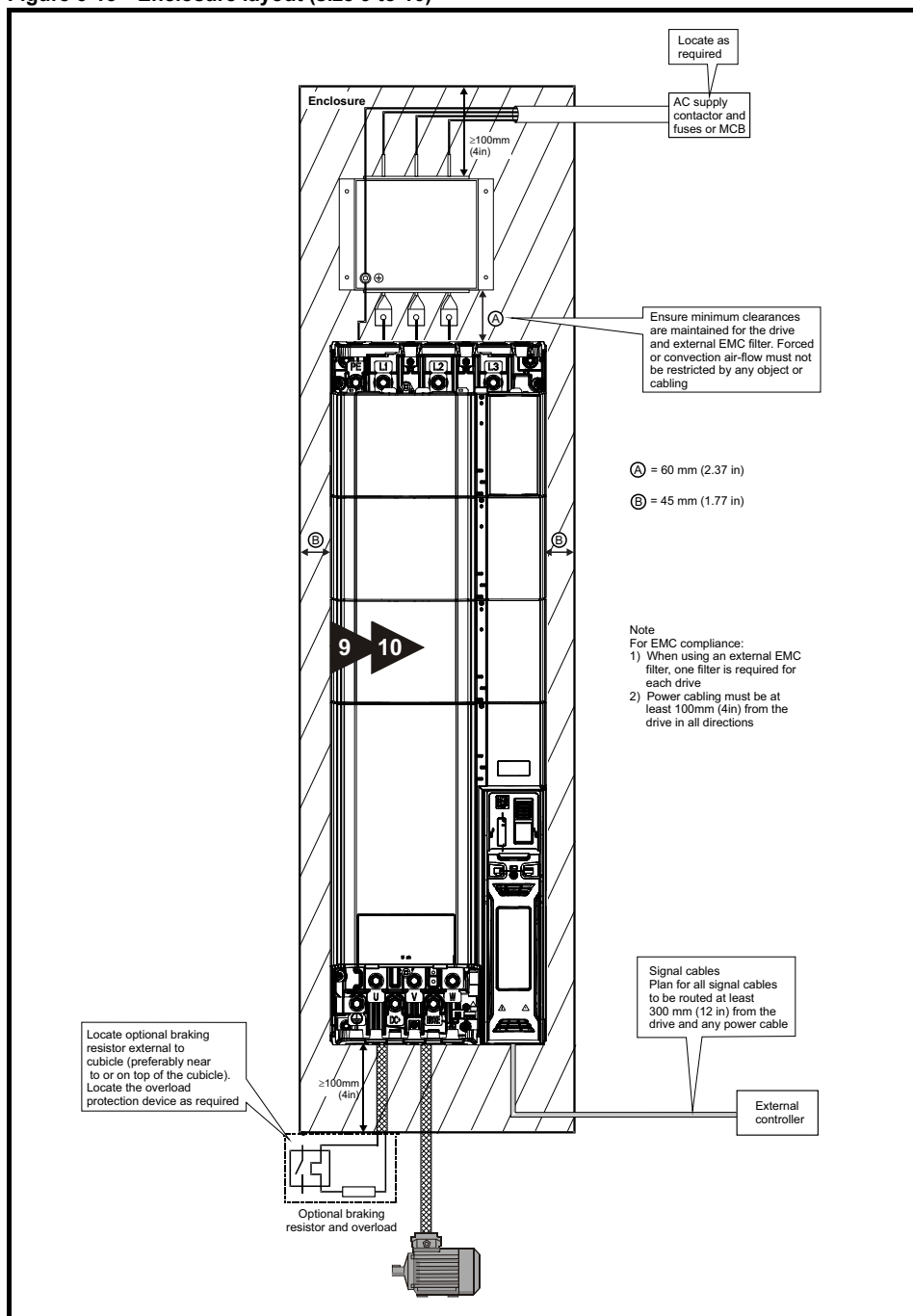
Figure 3-13 Enclosure layout (size 9 to 10)
