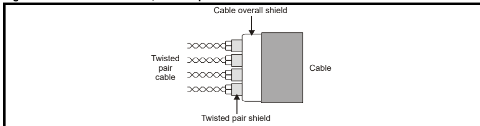
Figure 4-20 Feedback cable connections
