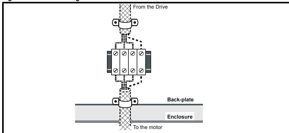
Figure 4-27 Connecting the motor cable to a terminal block in the enclosure
