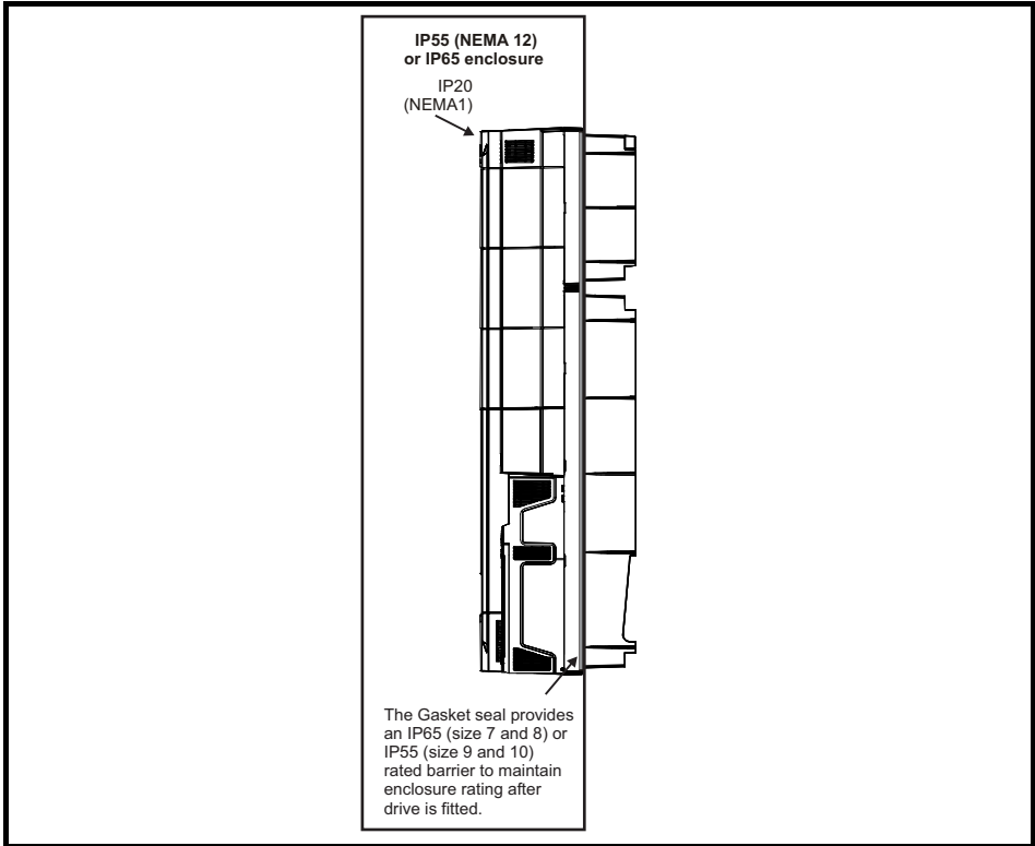
Figure 3-17 Example of high IP through-panel layout
