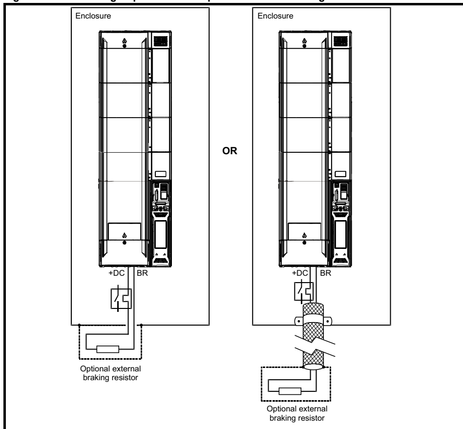
Figure 4-25 Shielding requirements of optional external braking resistor
