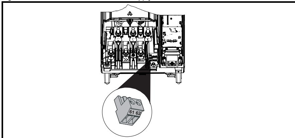
Figure 4-8 Location of the heatsink fan supply connector on size 9 to 10
