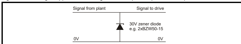
Figure 4-30 Surge suppression for analog and bipolar inputs and outputs
