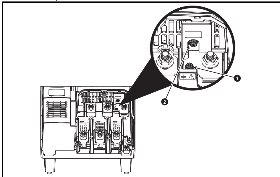
Figure 4-15 Removal of the size 7, 8 and 9A internal EMC filter and line to ground varistors (size 7 shown)
