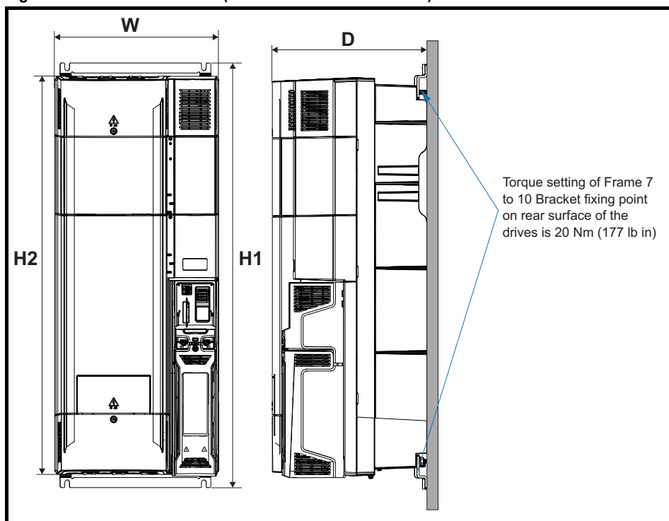
Figure 3-8 Drive dimensions (Unidrive M700 size 8 shown)
