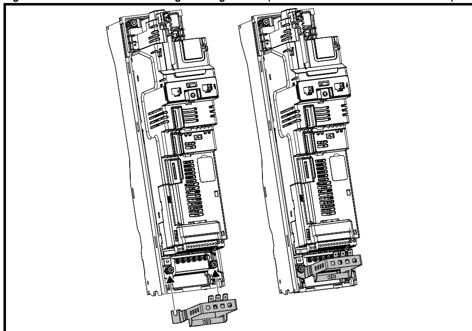
Figure 4-14 Installation of control grounding bracket (all sizes -Unidrive M700 size 3 shown)
