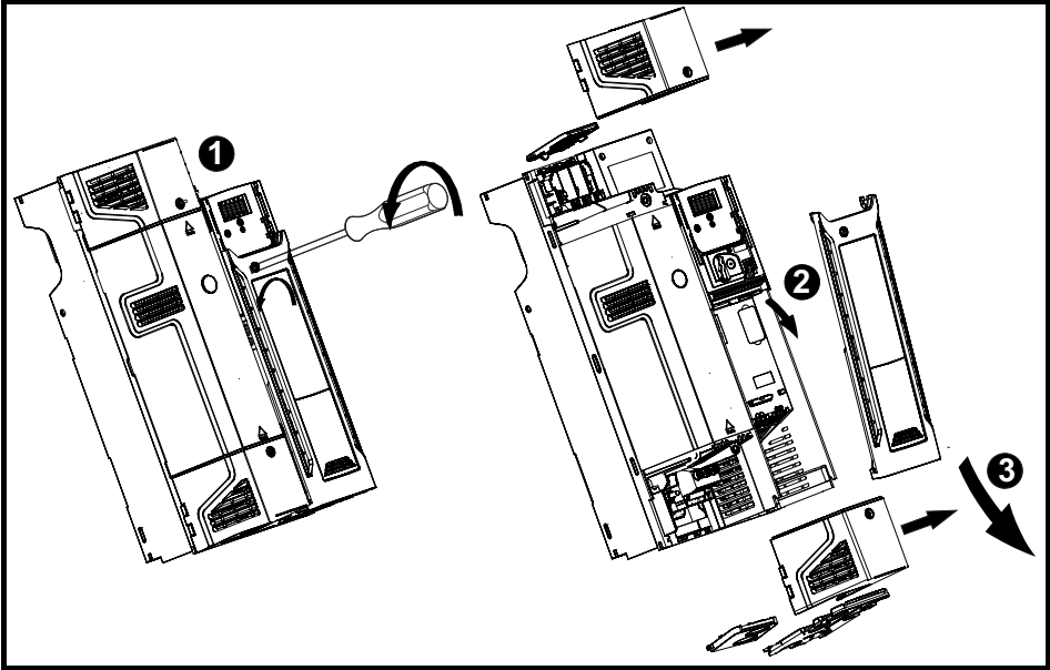
Figure 3-5 Removing the Unidrive M400 terminal cover
