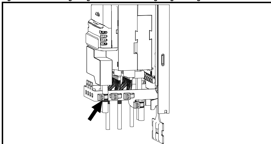
Figure 4-26 Grounding of signal cable shields using the grounding bracket
