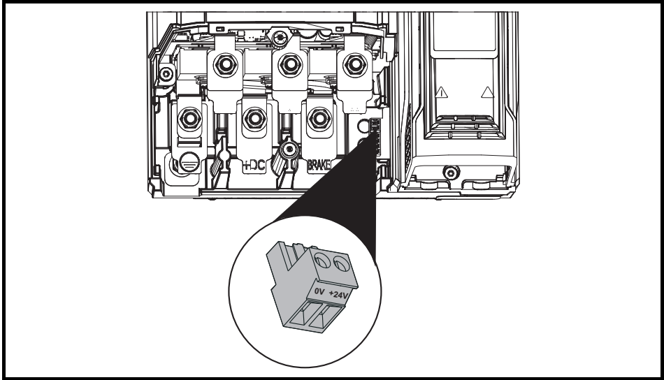
Figure 4-6 Location of the 24 Vdc power supply connection on size 7
