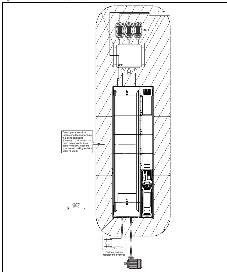
Figure 4-18 Drive cable clearances
