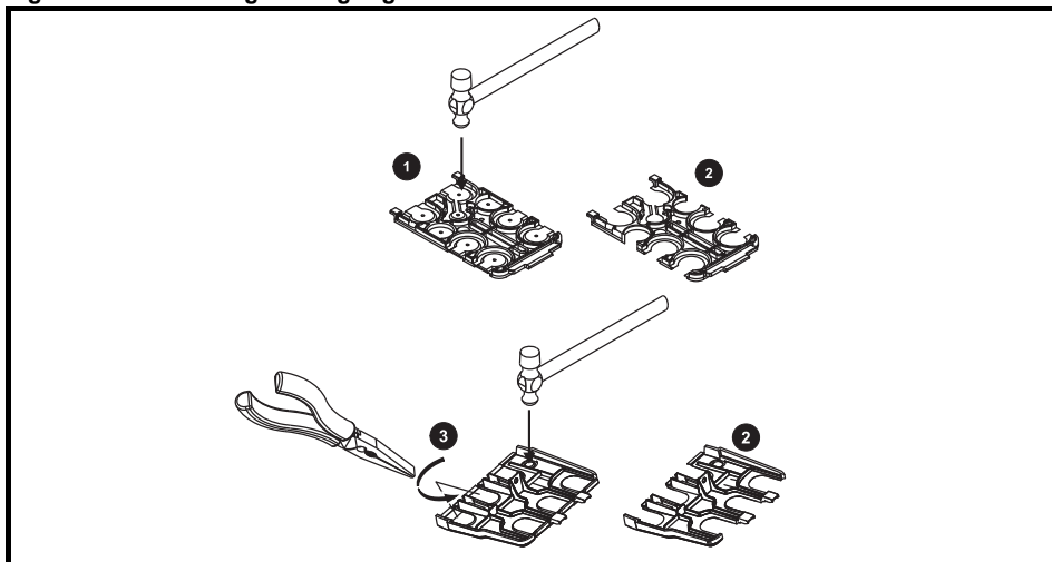
Figure 3-6 Removing the finger-guard break-outs
