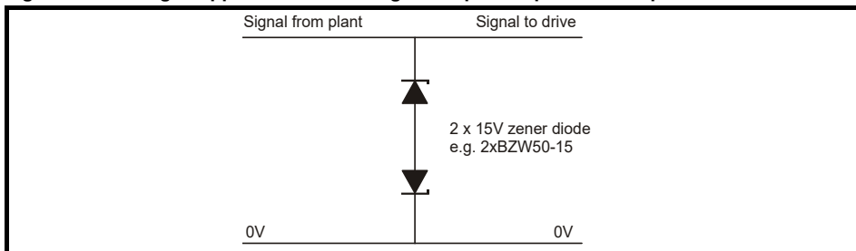
Figure 4-30 Surge suppression for analog and bipolar inputs and outputs
