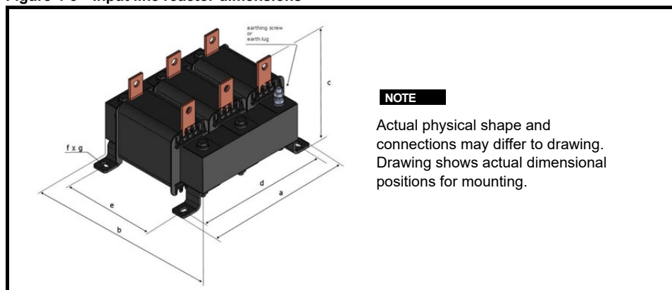
Figure 4-5 Input line reactor dimensions
