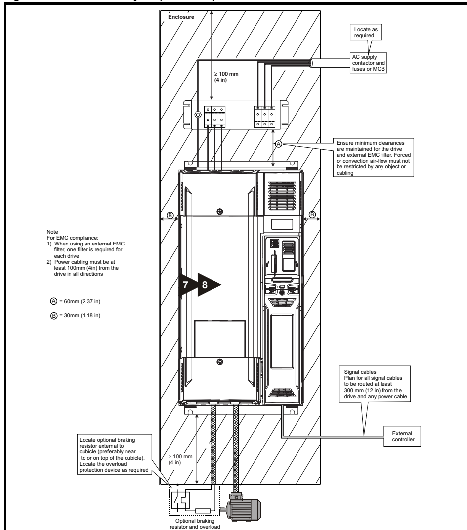
Figure 3-12 Enclosure layout (size 7 to 8)
