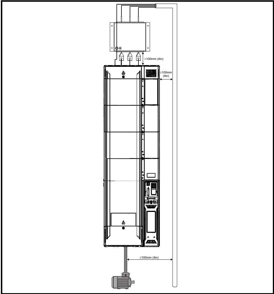
Figure 4-21 Supply and ground cable clearance
