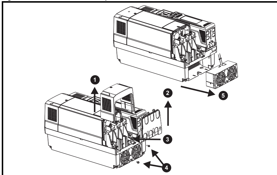
Figure 3-24 Size 7 heatsink fan replacement
