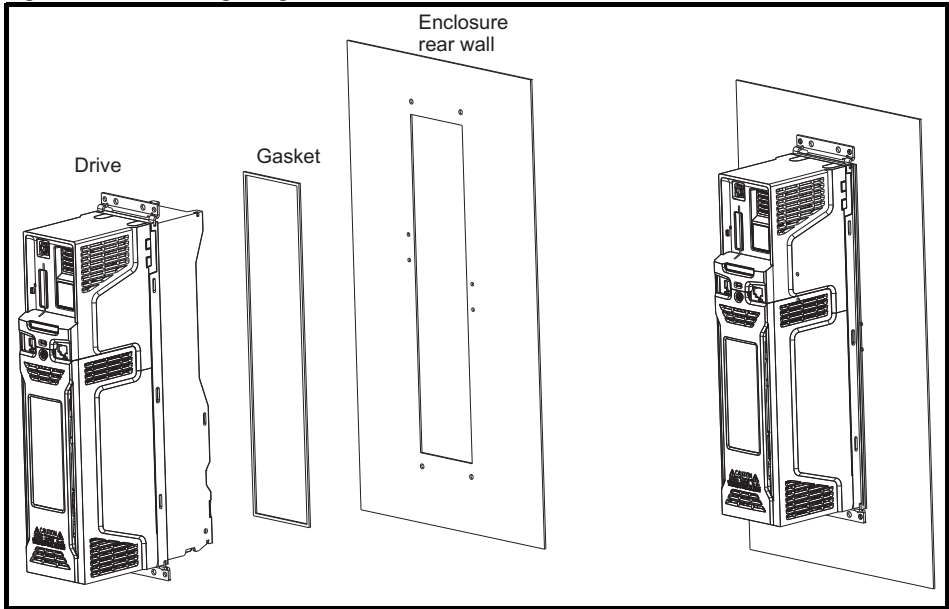
Figure 3-15 Installing the gasket
