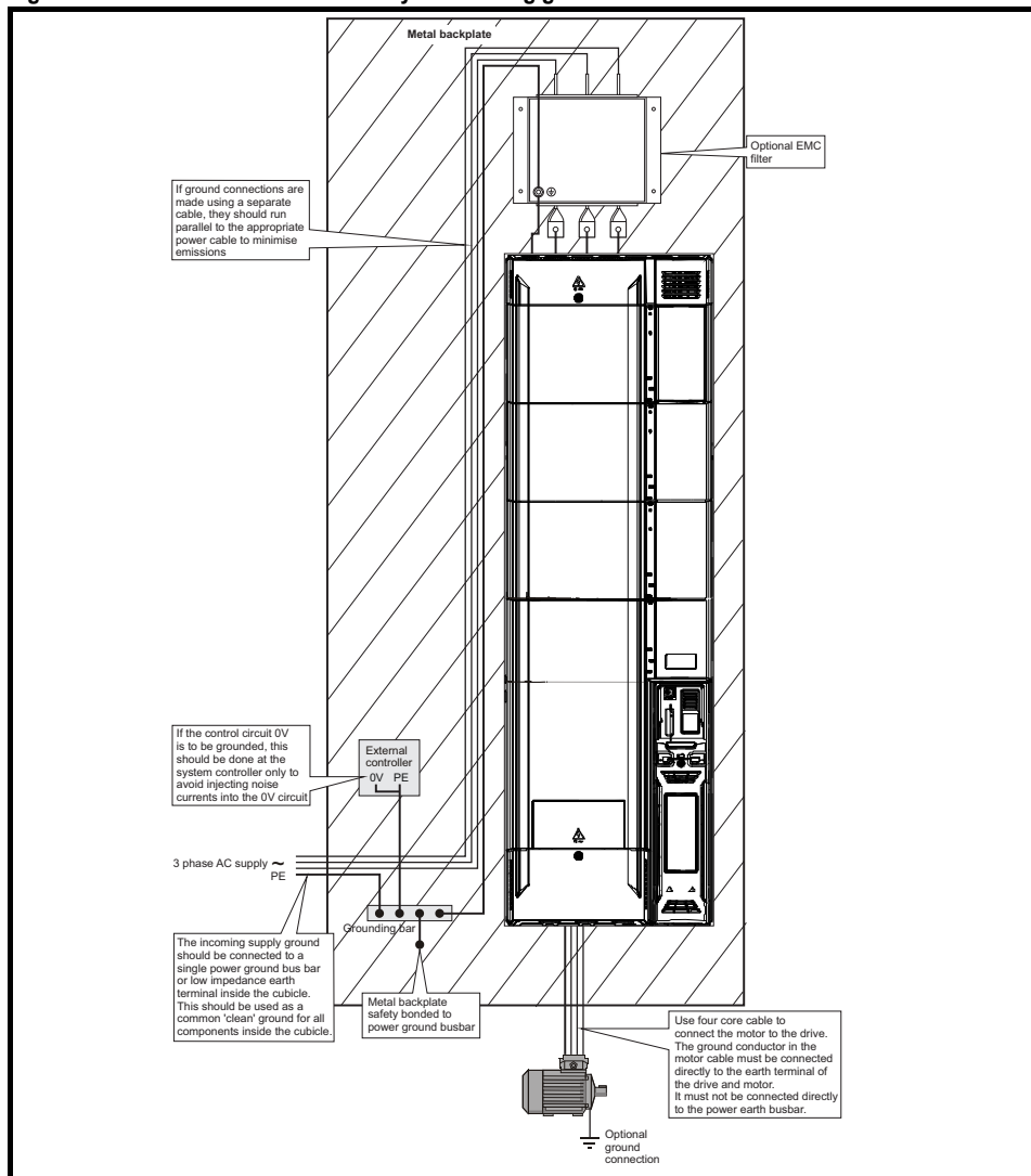
Figure 4-17 General EMC enclosure layout showing ground connections
