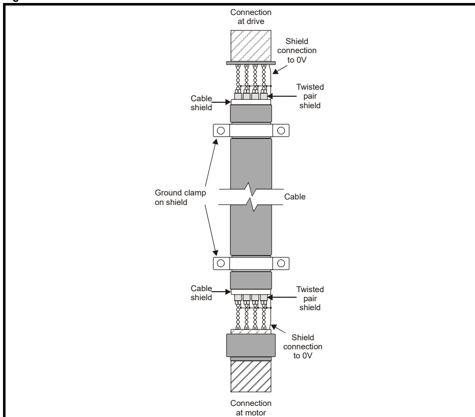
Figure 4-20 Feedback cable connections
