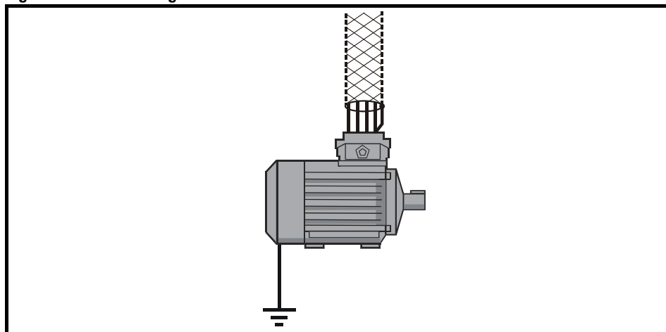
Figure 4-24 Grounding the motor cable shield
