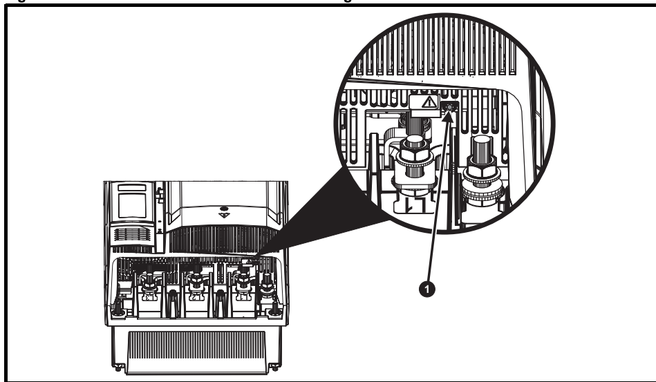
Figure 4-16 Removal of size 9E and 10E line to ground varistors
