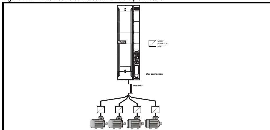
Figure 4-11 Alternative connection for multiple motors
