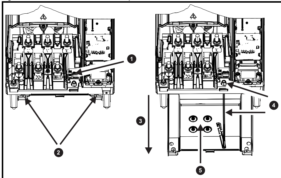
Figure 3-26 Size 9 and 10 heatsink fan replacement
