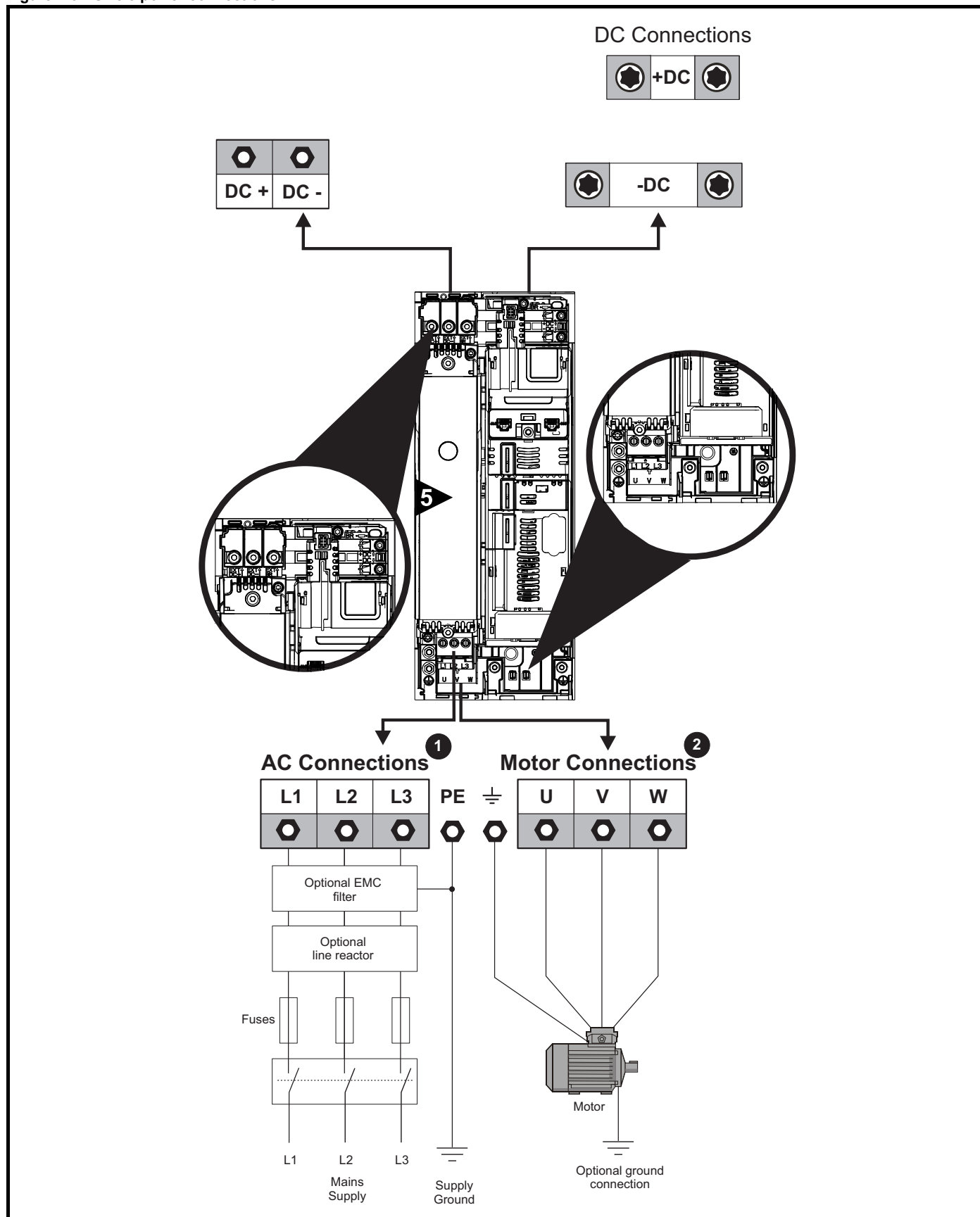
Figure 4-3 Size 5 power connections
