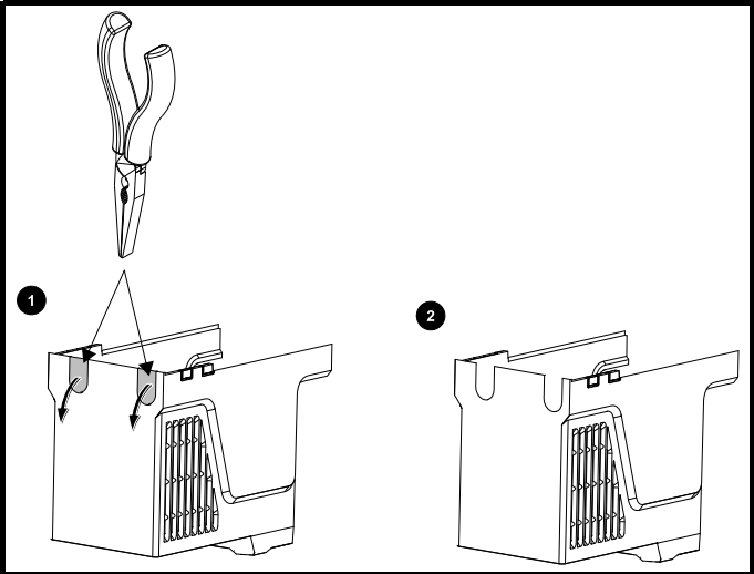
Figure 3-12 Removing the size 3 and 4 DC terminal cover break-outs
