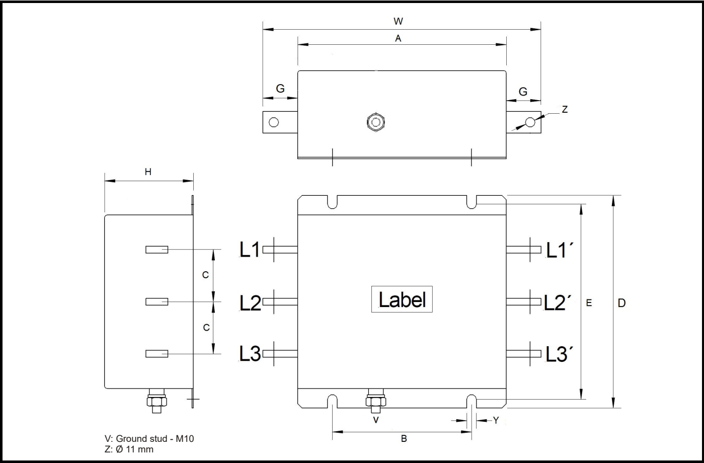
Figure 3-56 External EMC filter (size 9E and 10)
