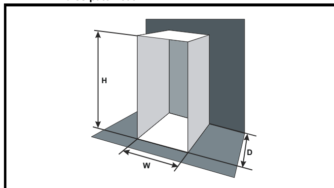
Figure 3-41 Enclosure having front, sides and top panels free to dissipate heat
