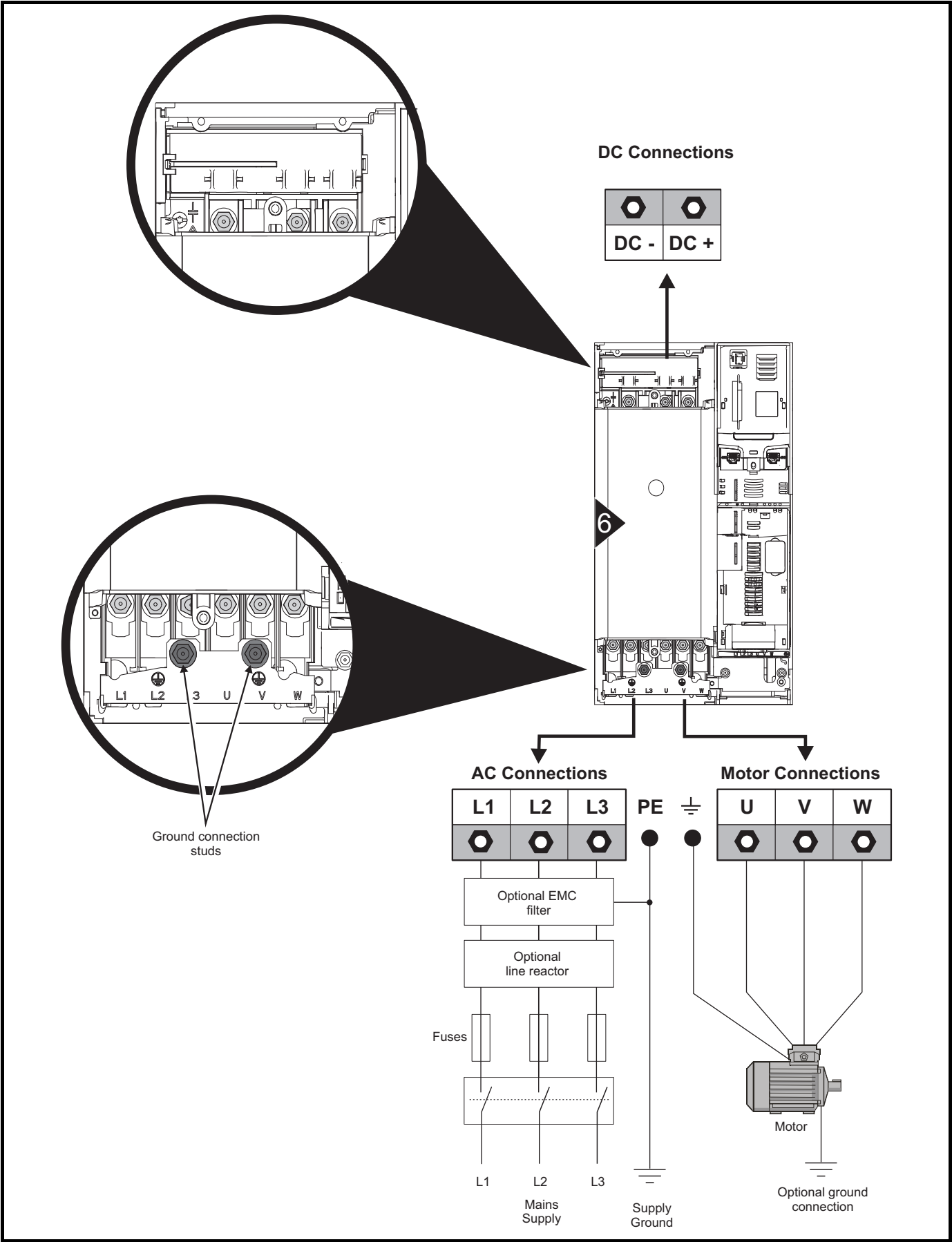
Figure 4-4 Size 6 power connections
