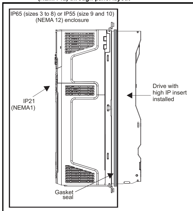
Figure 3-42 Example of IP65 (sizes 3 to 8) or IP55 (size 9 and 10) (NEMA 12) through-panel layout
