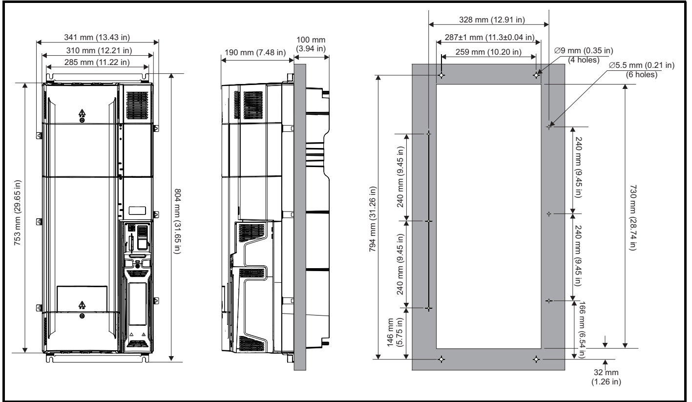
Figure 3-30 Through panel mounting the size 8 drive
