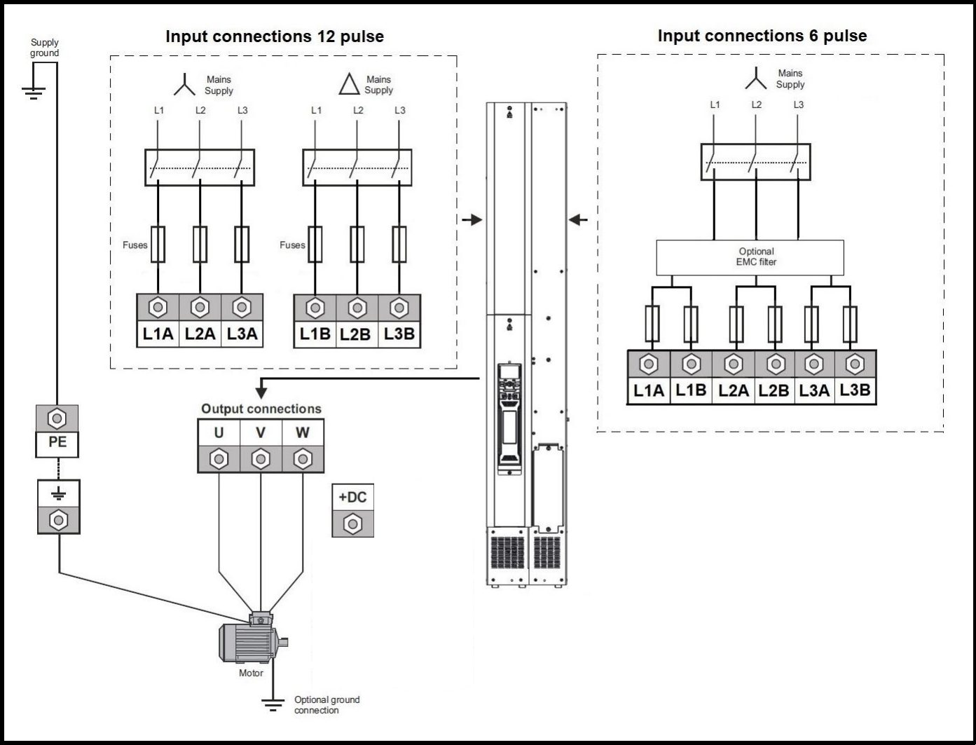
Figure 4-8 Power Module Frame 12 power connections
