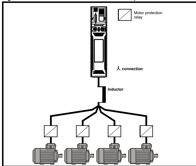
Figure 4-24 Alternative connection for multiple motors
