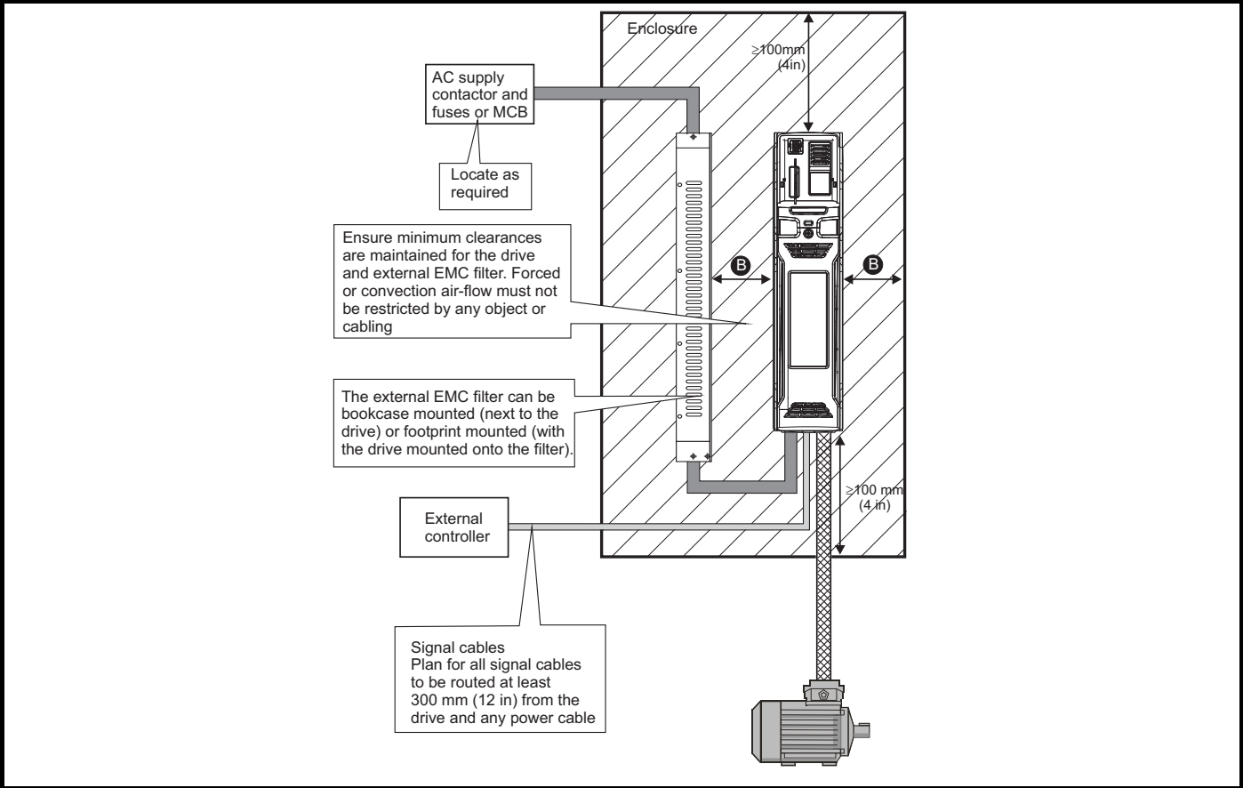
Figure 3-39 Enclosure layout (size 3 to 8)
