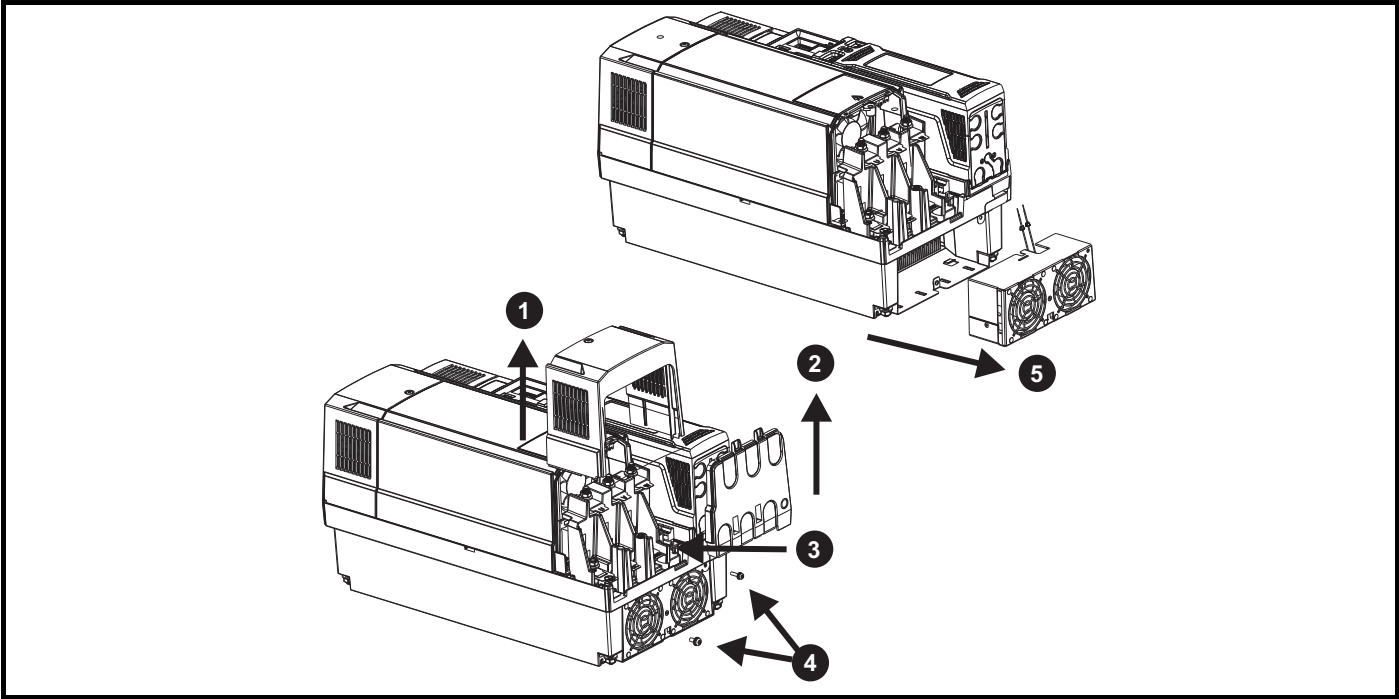
Figure 3-67 Size 7 heatsink fan replacement
