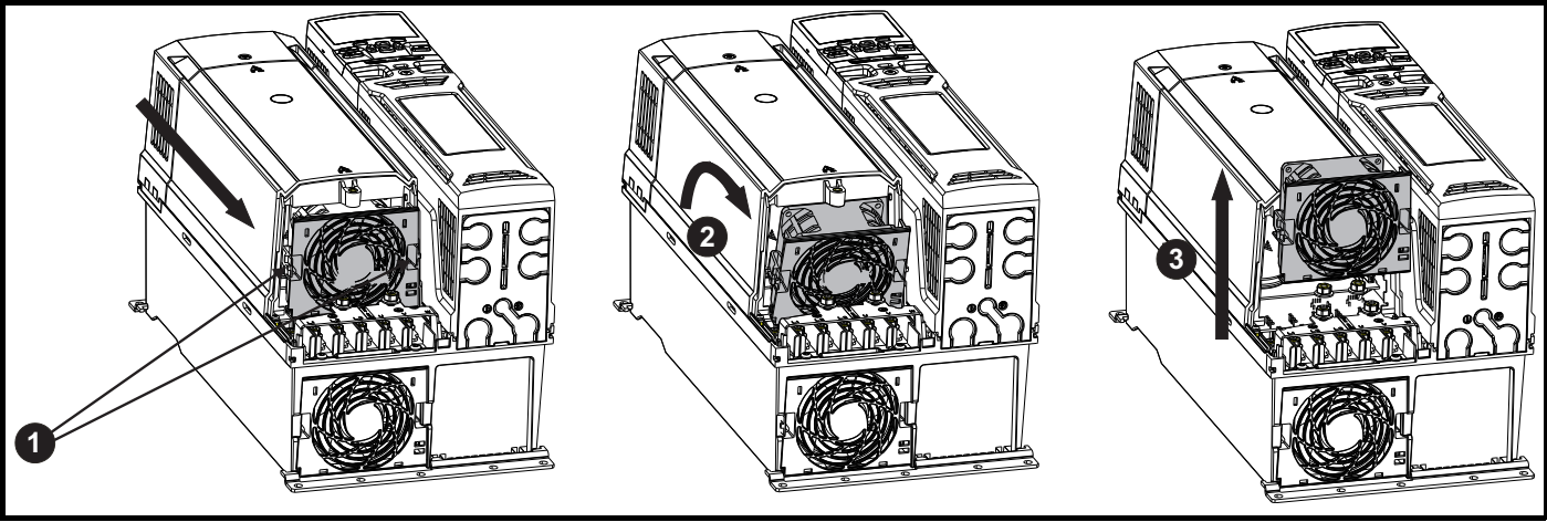
Figure 3-70 Removal of the size 6 auxiliary(capacitor bank) fan
