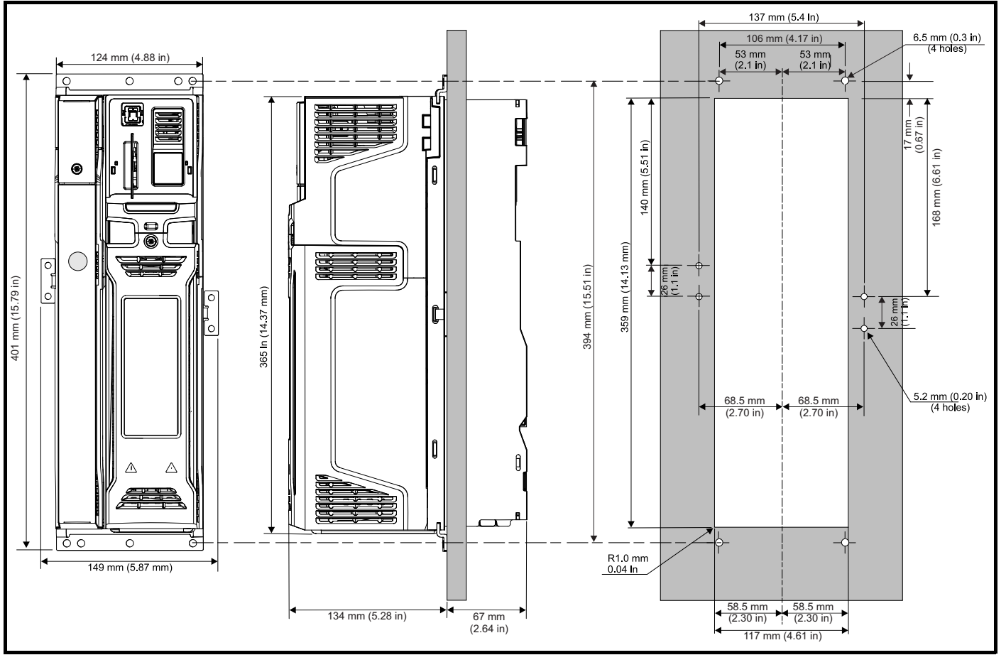
Figure 3-27 Through panel mounting the size 5 drive
