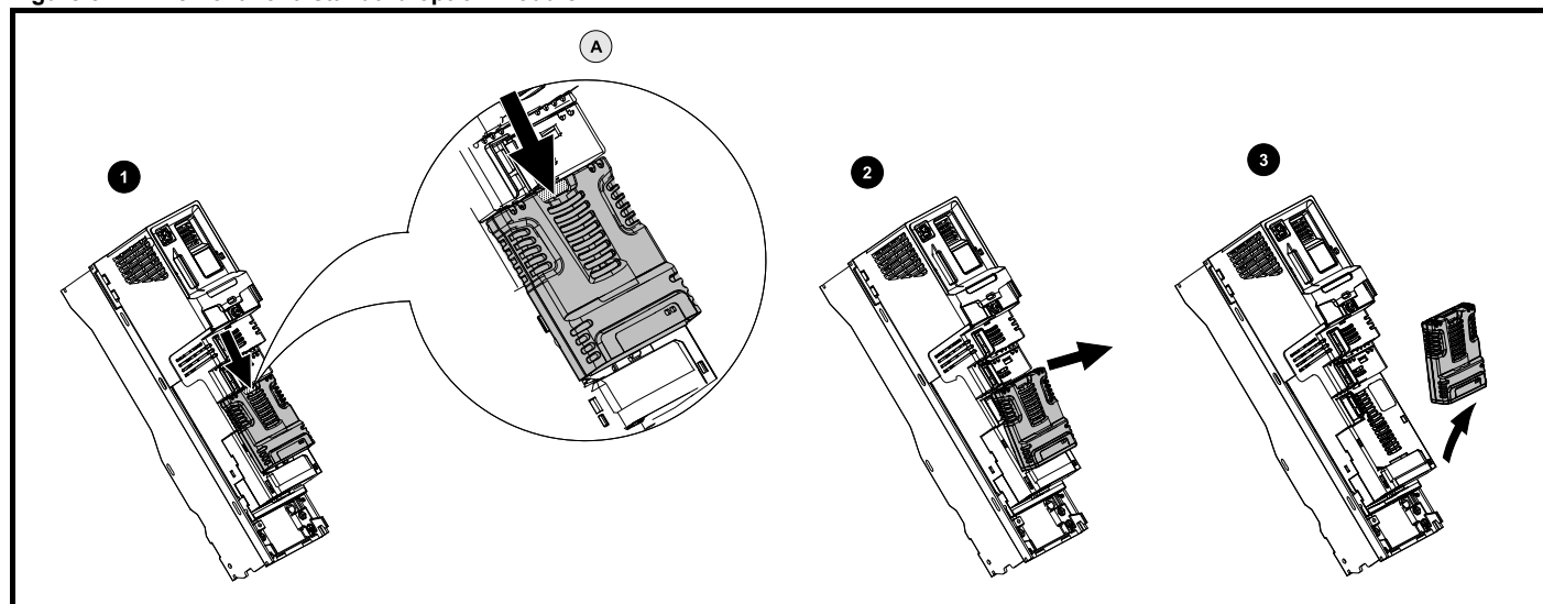
Figure 3-14 Removal of a standard option module
