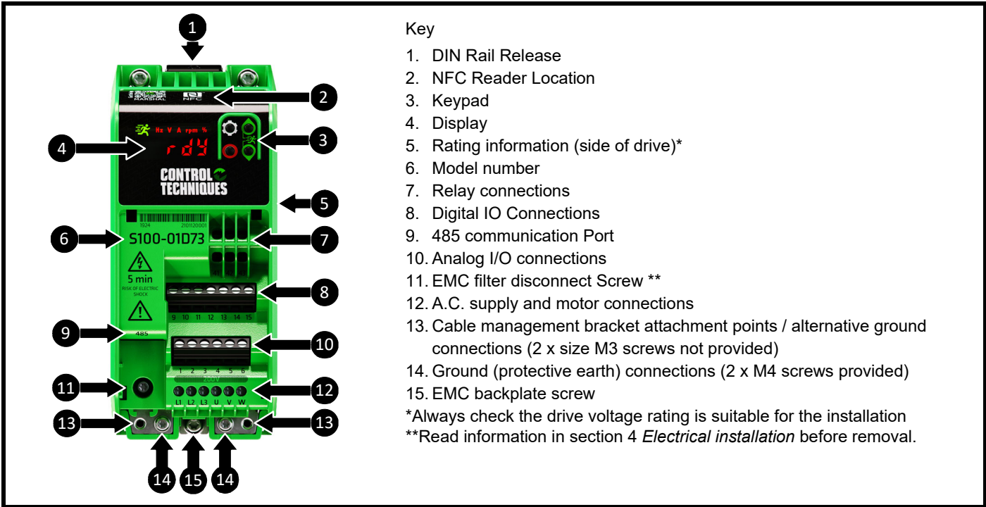
Figure 2-4 Features of the drive
