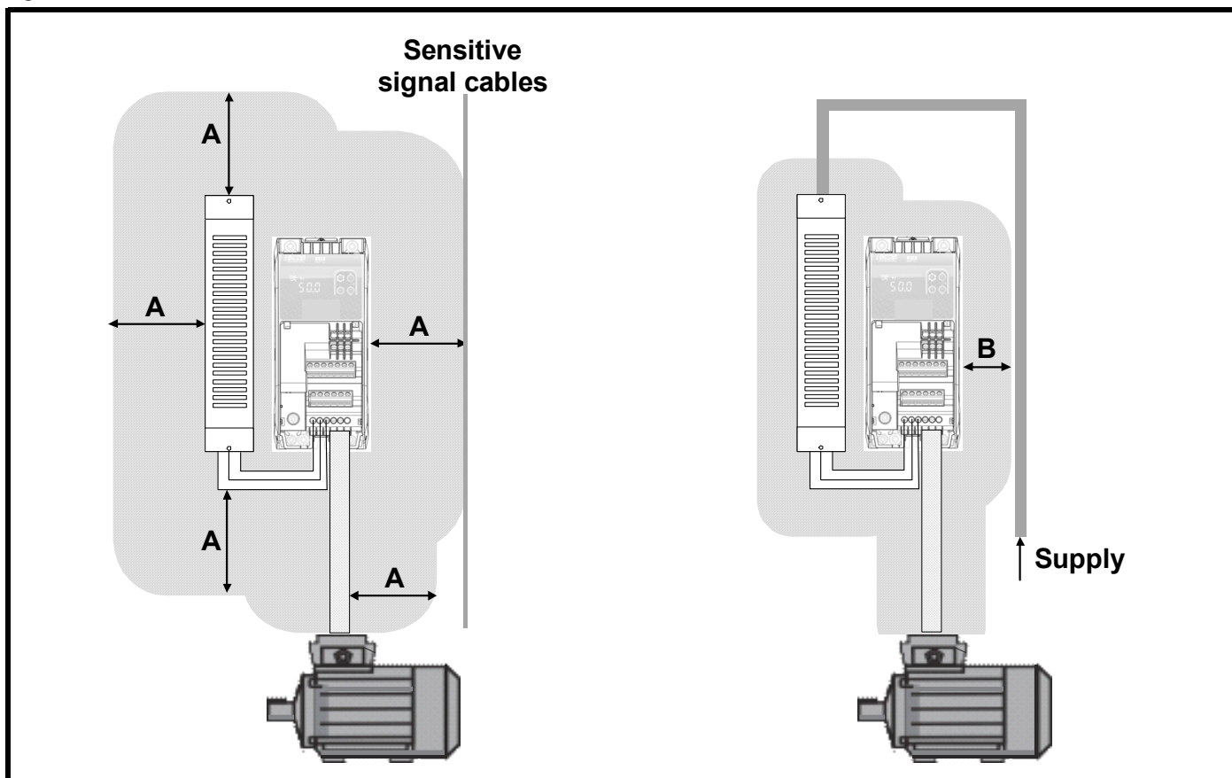
Figure 4-9 Suitable cable clearances
