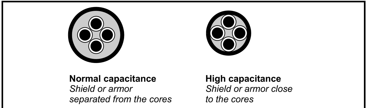
Figure 4-4 Cable construction influencing the capacitance
